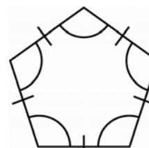
regular polygon
